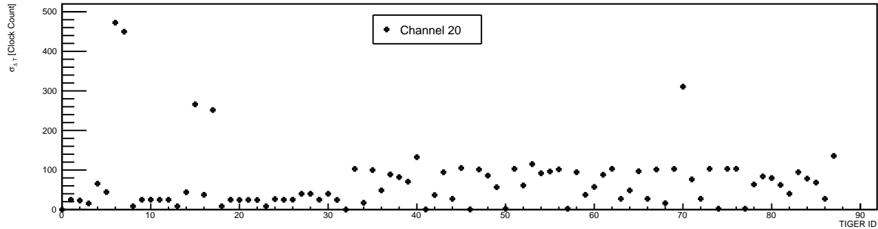
i-th TIGER \sigma_{\Delta T} per Channel
